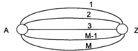
Fig. 7 Nodes A and Z between which traffic T flows over M disjoint paths.
