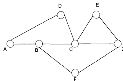
Fig. 2 The simple approach algorithm fails to produce a vertex-disjoint pair of paths between A and Z.
